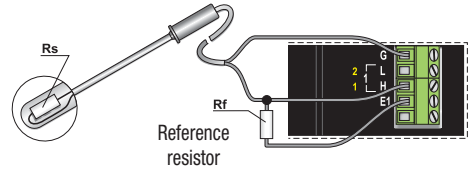
2-WIRE RESISTIVE SENSORS
