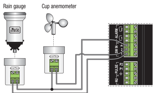
Sensors with contact frequency output
