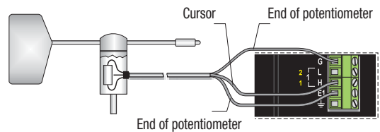
3-wire potentiometric sensors
